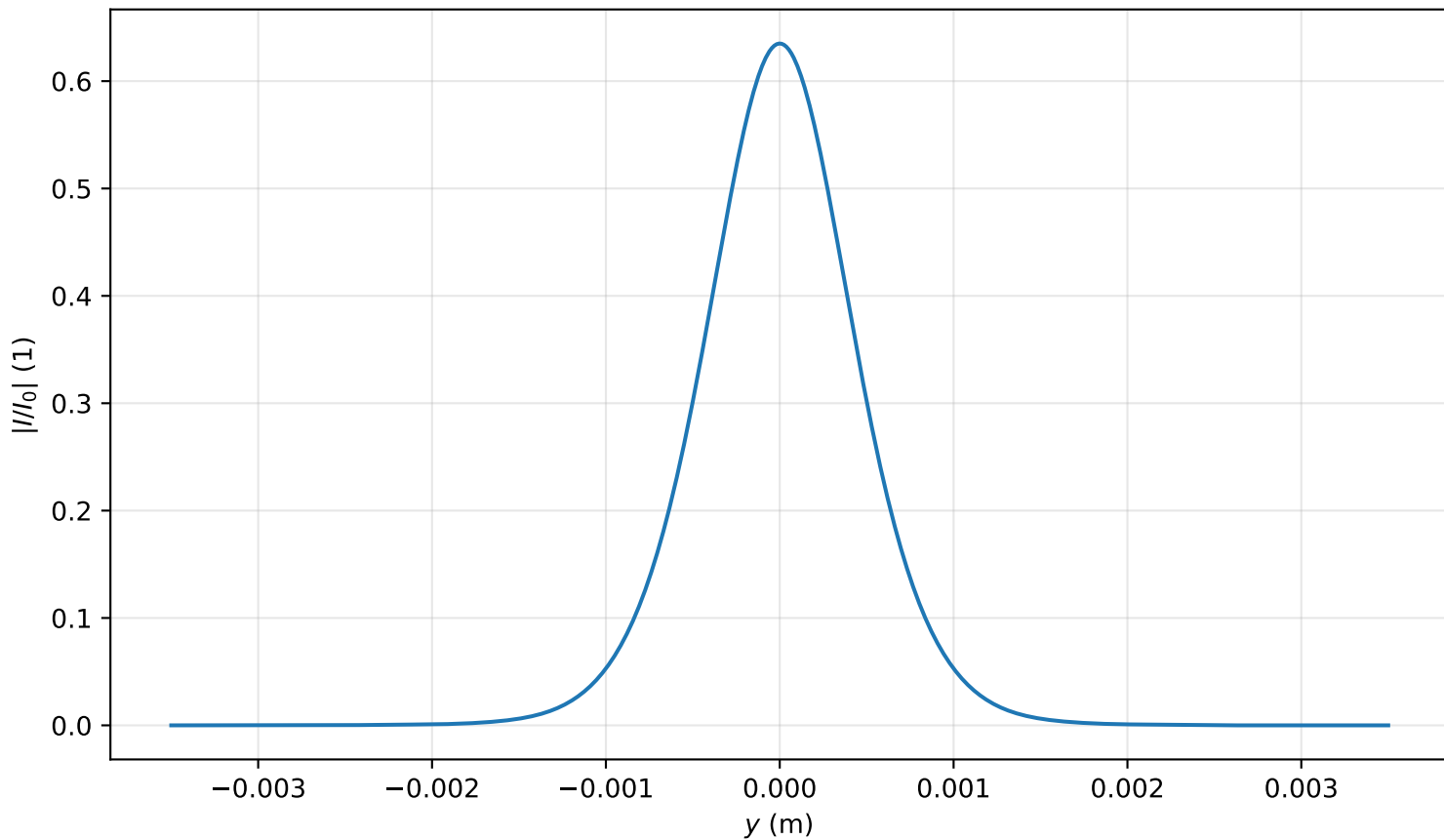
Intensity profile I(x=0, y, z=3.184)/I_0 , P_{in}=0.6P_{cr} , artificial time
